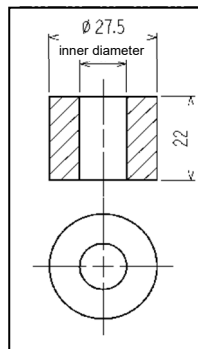
Rubber seal
